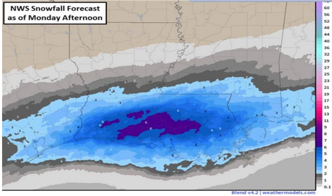
NWS snowfall forecast model across Louisiana as of Monday Afternoon Photo credit: weathermodels.com by weather.us
